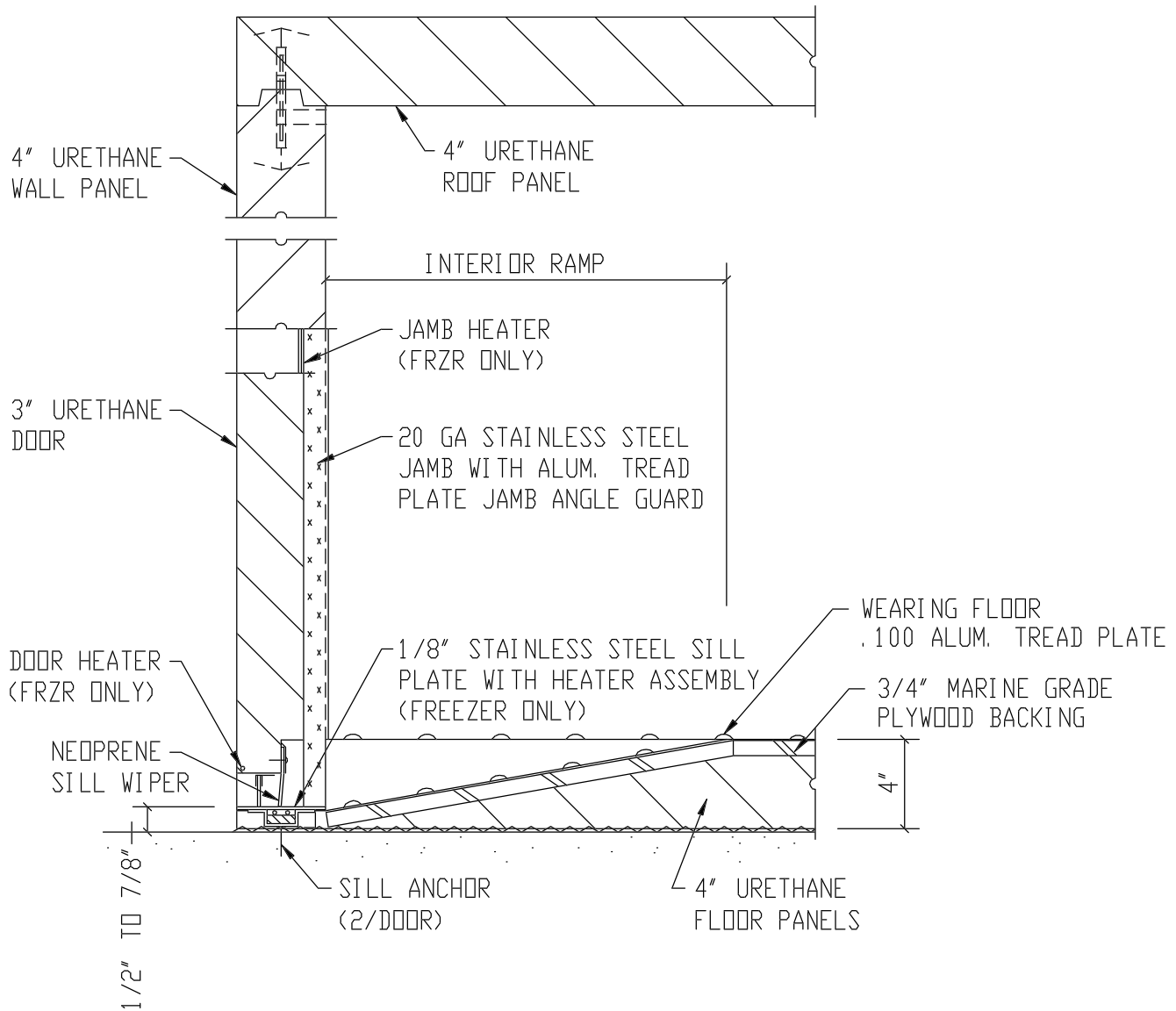
SECTION (@ DOOR) 1-1/2" = 1'-0" (FP)
