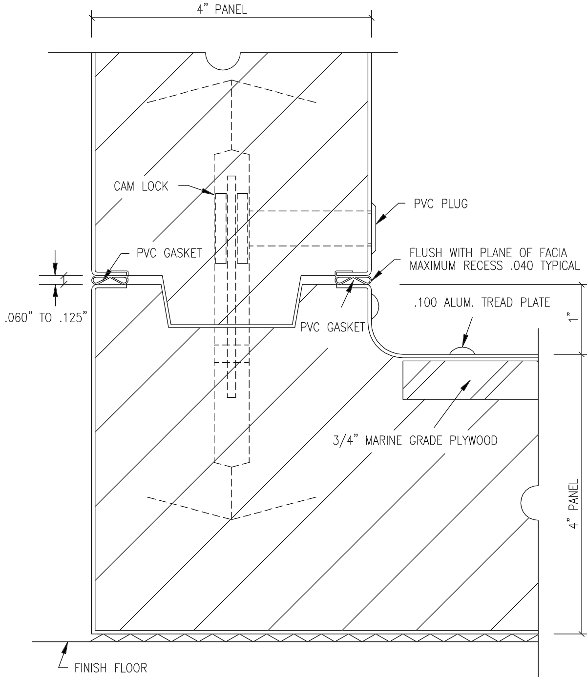
TYPICAL SECTION JOINT DETAIL
