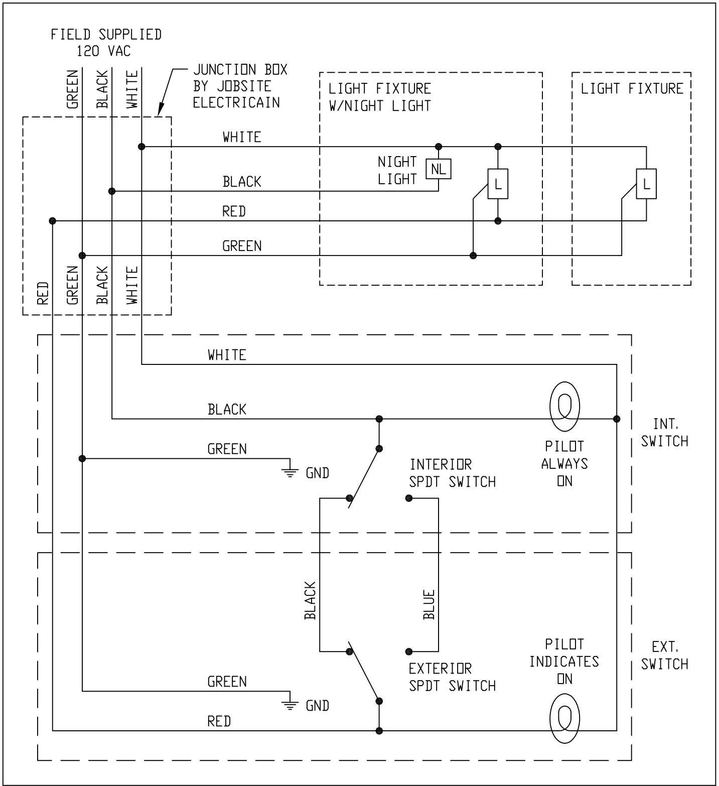
SINGLE ENTRANCE LIGHT CONTROL WIRING DIAGRAM
